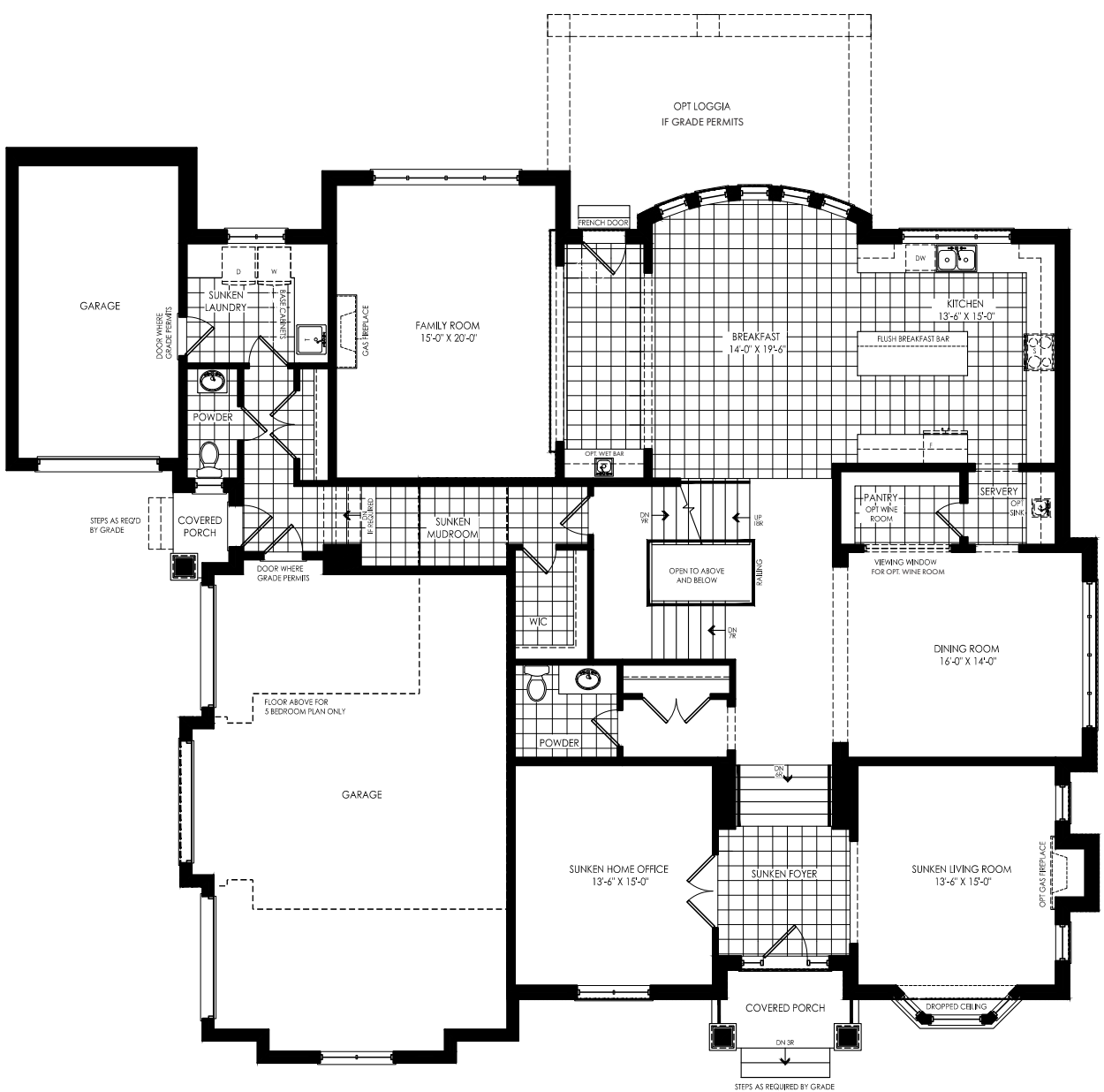
MAIN FLOOR ELEVATION B
